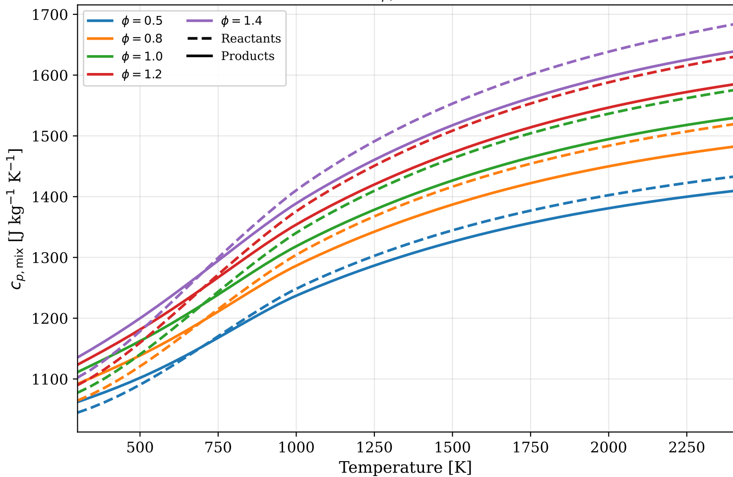
Mixture c_{p,\text{mix}} — \text{CH}_4/\text{air}
